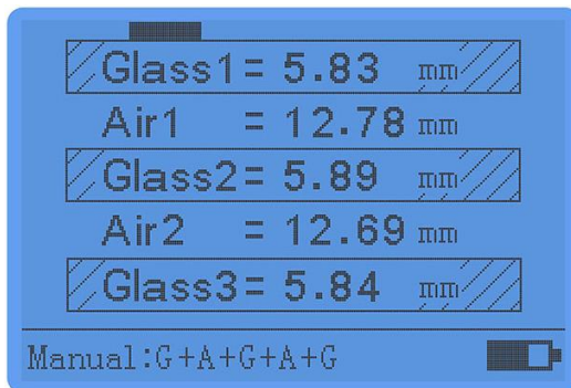
Triple glazing
