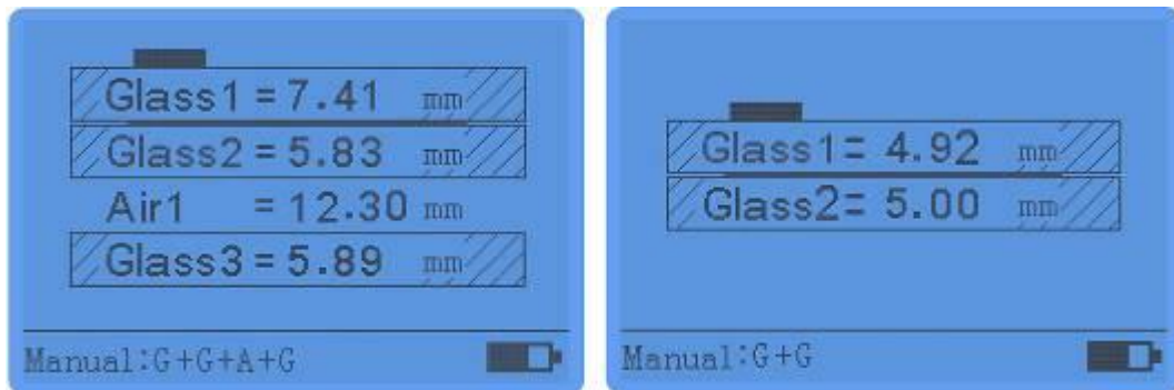
Laminated glass with one layer air
