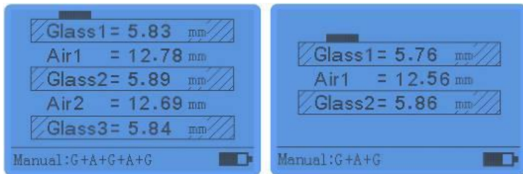
Triple glazing
